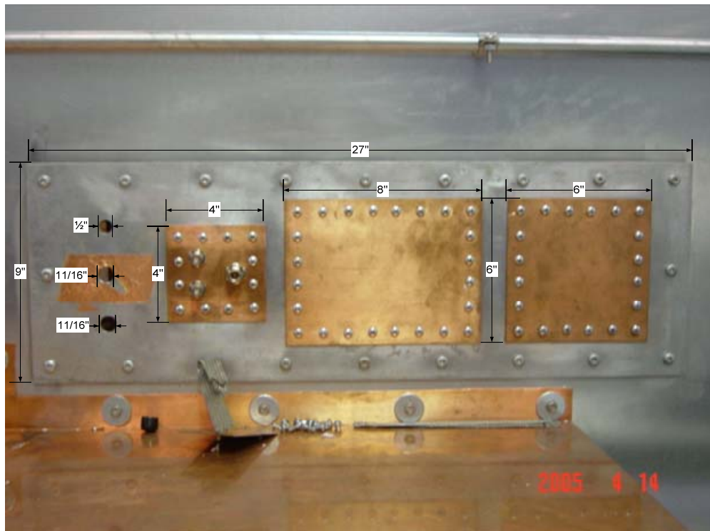
FIG-5: Room 27P Waveguide Cover Plate (Monitor Room)
