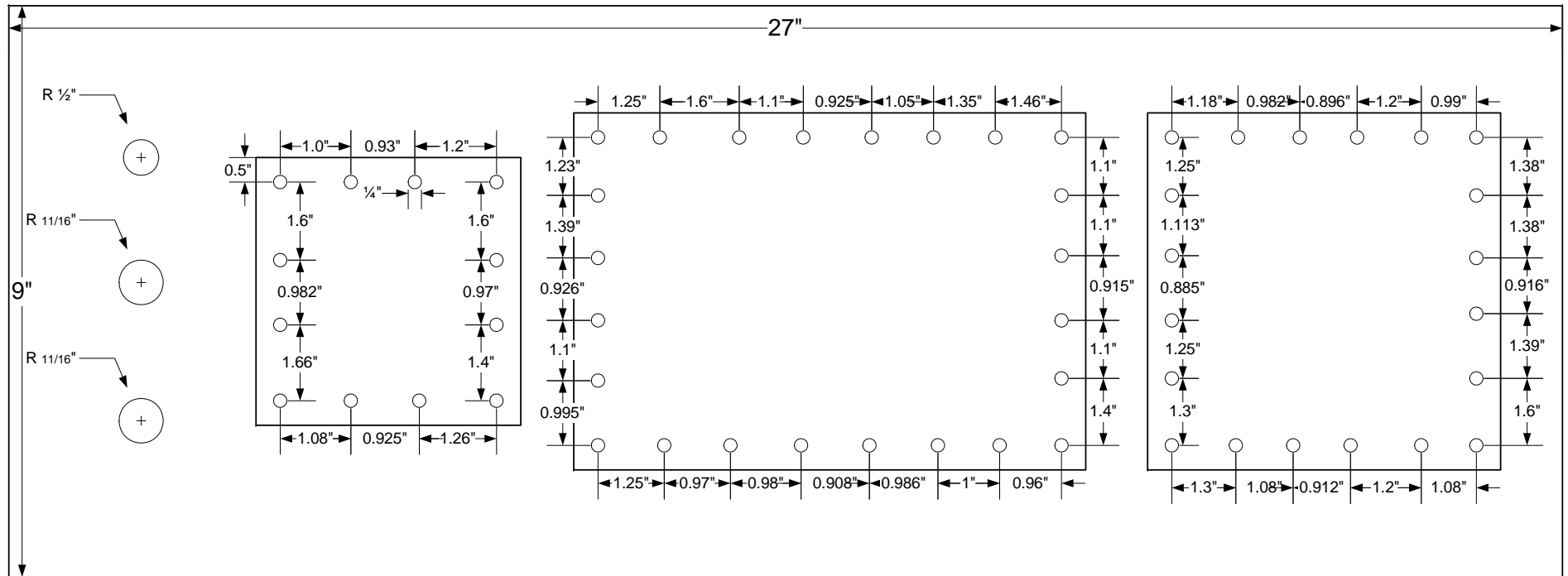
FIG-6: Room 27P Waveguide Cover Plate Dimensions (Monitor Room)
