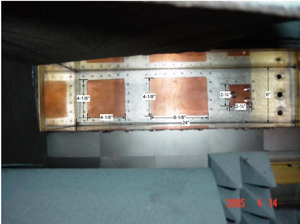
FIG-4: Room 27U Waveguide Extension Opening (Back of Plate)
