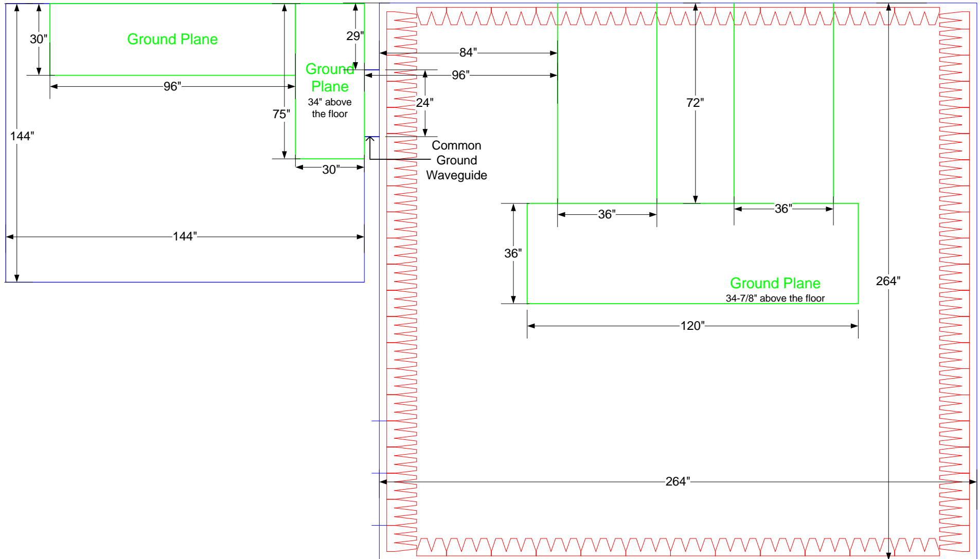
Fig-3: Rooms 27U (Test Room) & 27P (Monitor Room)
